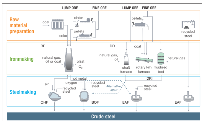
Figure 1: Steelmaking routes
