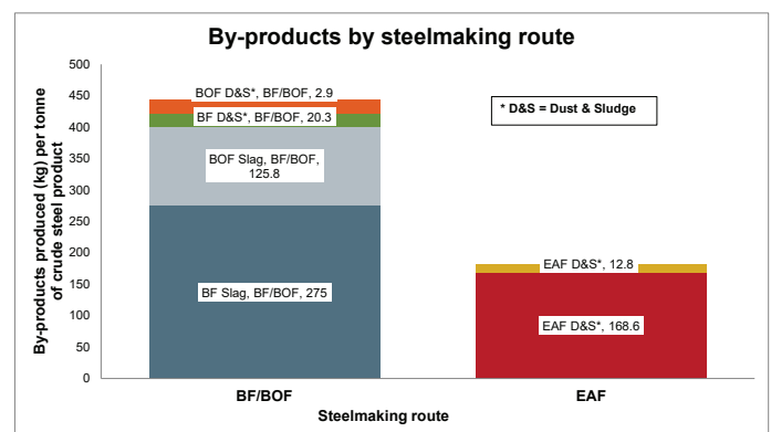
Figure 1: Main solid co-products by steelmaking routes 2
