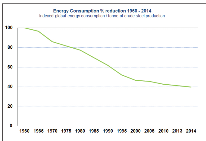
Figure 1: Indexed global energy consumption/tonne of crude steel production
